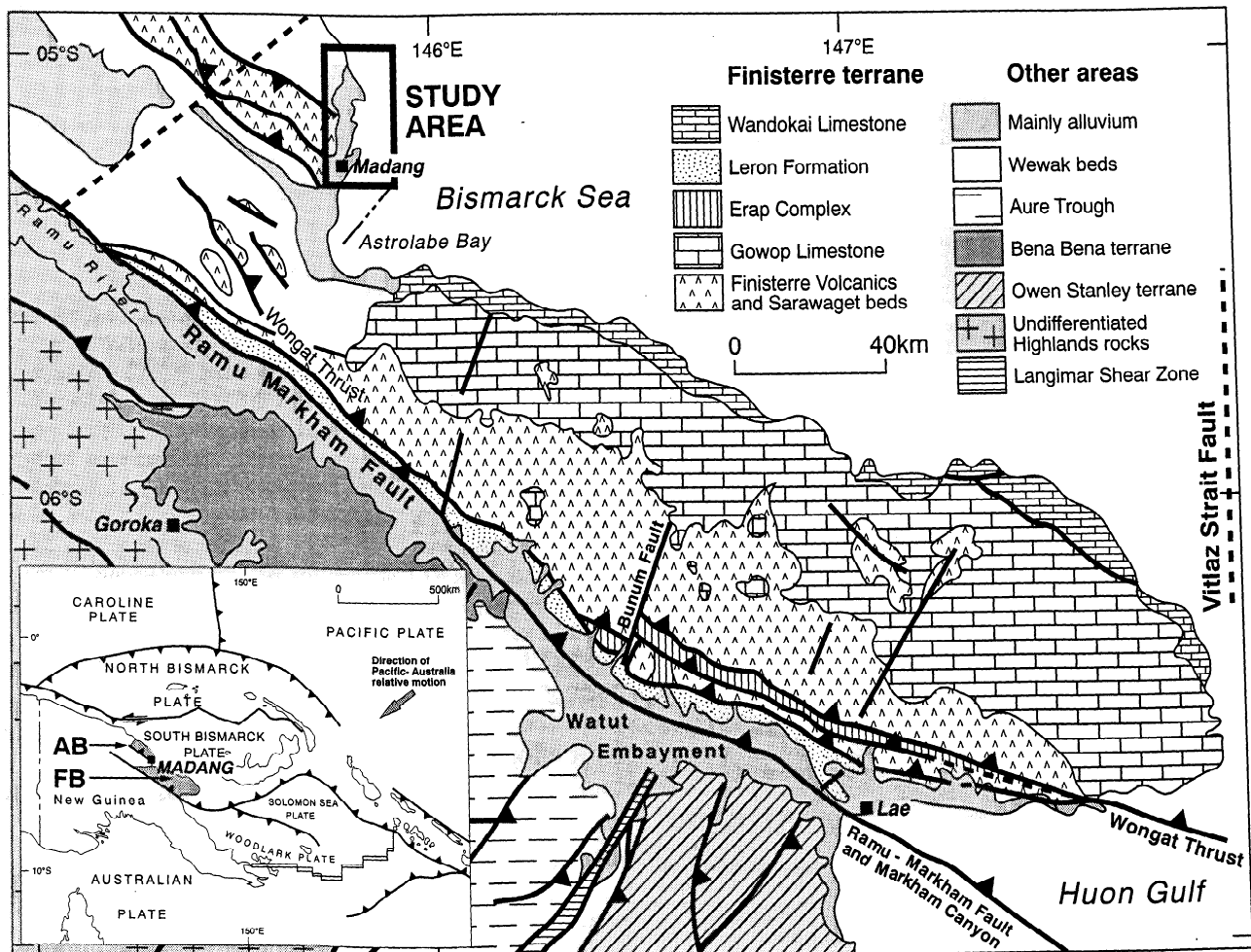
Figure 1. Tectonic setting of the study area, north coast of Papua New Guinea. In the inset, the Adelbert block and the Finisterre block of the Finisterre Terrane are shown in heavy shading and labeled with AB and FB, respectively. In the main figure (based on Abbott et al. [1994]), heavy solid lines are faults with barbs on the upper plate of thrusts, the NE and north trending dashed lines are seismically active strike-slip faults, and the dash-dotted line in Astrolabe Bay marks a postulated NE trending cross fault that is presumed to have ruptured during the 1970 Madang earthquake [Everingham, 1975; Abers and McCaffrey, 1994]. Inset figure is based on Tregoning et al. [1998].
