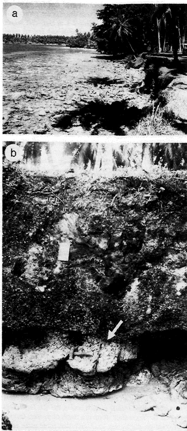
Figure 3. (a) The present-day reef flat and the lower coastal cliff and terrace at Jais Aben. Note the evidence of active erosion of the cliff, which, combined with the relatively narrow reef flat (~30-40 m wide), lends support to the concept of a major tectonic uplift event within the past few centuries. (b) Lower coastal cliff at Jais Aben. Massive Porites coral microatolls of 1-2 m diameter (e.g., under hammer) are abundant in a layer near the base of the cliff. The tops of these corals (e.g., arrow) form a distinctive boundary which is present throughout the field area. This boundary indicates the former position of sea level. Above the massive coral layer the cliff comprises a mixed branching and massive coral assemblage which indicates a rapid rise in relative sea level. Subsequent uplift has resulted in the present-day subaerial exposure of these reefs. (The hammer is 240 mm long.)
