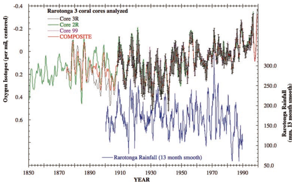
Fig. 4 Comparison of Rarotonga coral \delta^{18}\text{O} from 3 different cores from Porites lutea coral colonies to instrumental rainfall. The average \delta^{18}\text{O} over the interval from 1950 to 1997 was subtracted from each \delta^{18}\text{O} record and the centered series was then filtered with a 2-year smoothing spline filter. The three cores were used to make a composite \delta^{18}\text{O} record over the interval from 1997 to 2006 and a 2-core composite over the interval from 1906 to 1874. The composite \delta^{18}\text{O} record is shown in red. The standard deviation of the 3-core composite is also shown. The rainfall data was smoothed with a 13 month running average filter to highlight interannual and interdecadal variability
