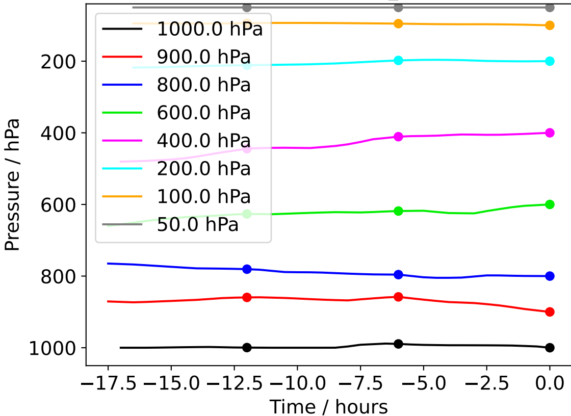
Camborne 20260108_000000
