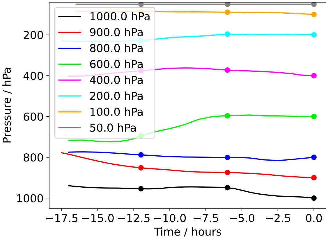
Camborne 20260107_060000
