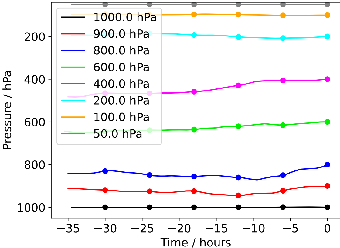
Camborne 20240725_120000
