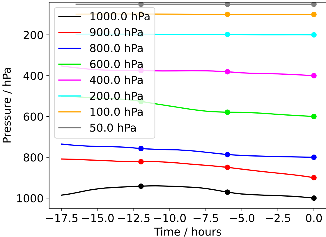
Camborne 20240608_180000
