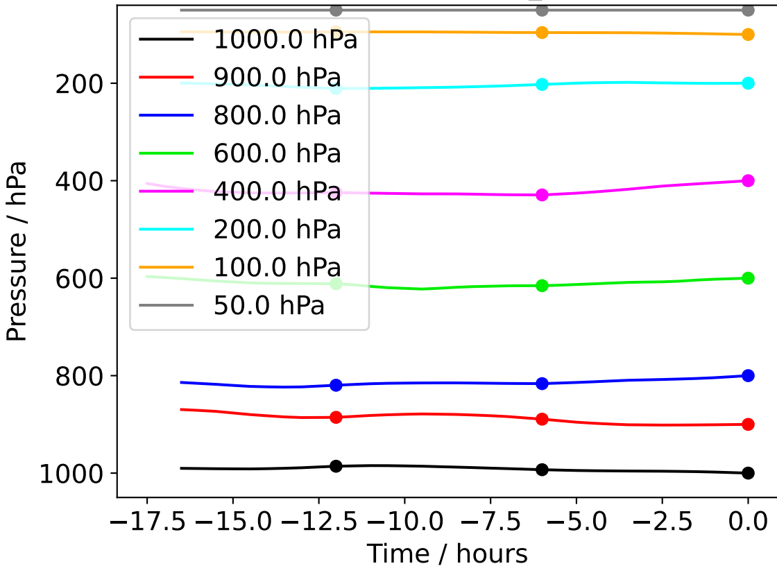
Camborne 20240414_120000
