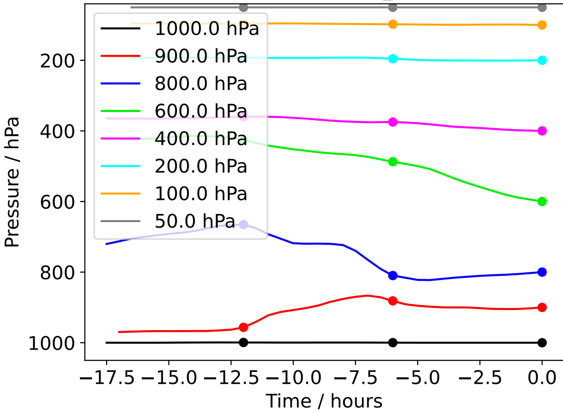
Camborne 20240408_180000
