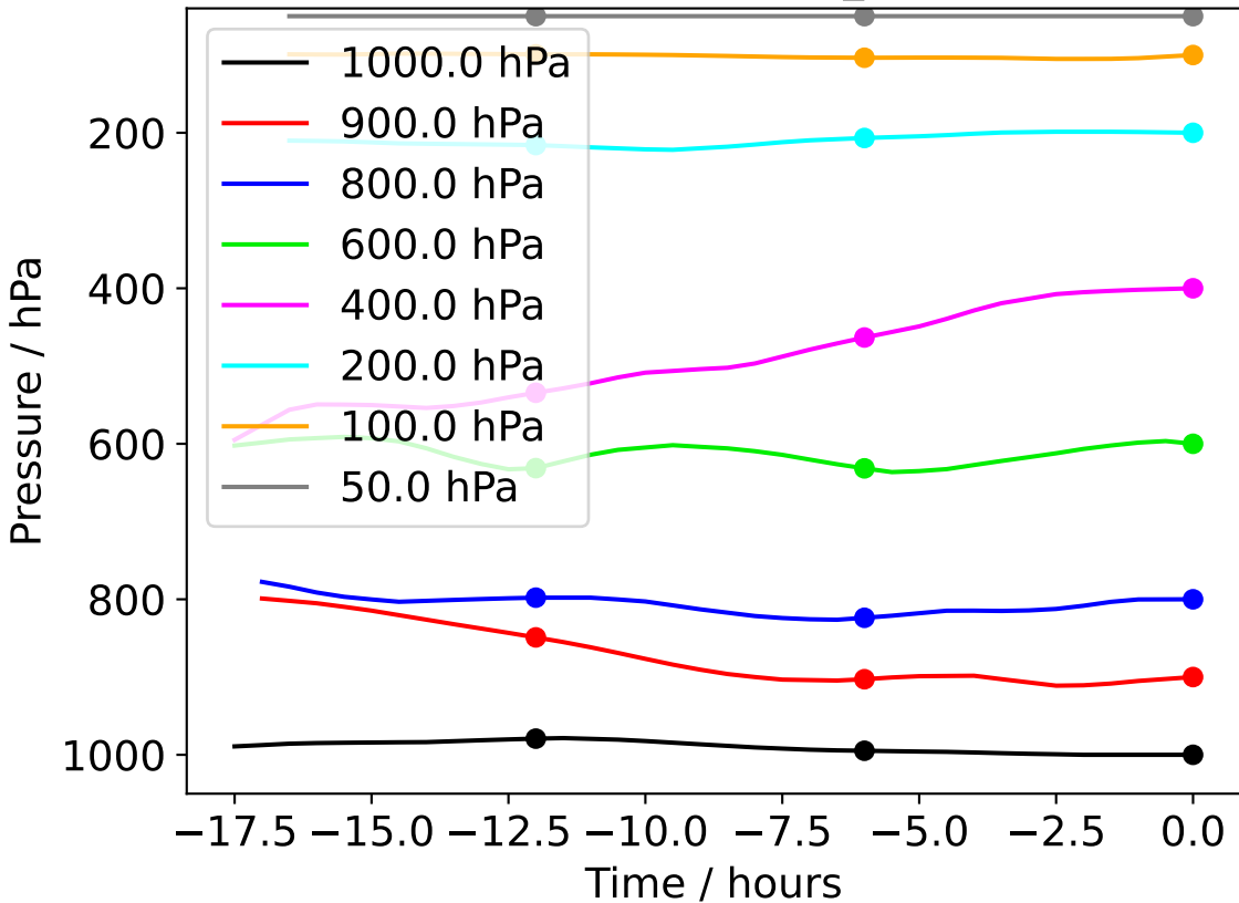
Camborne 20240217_120000
