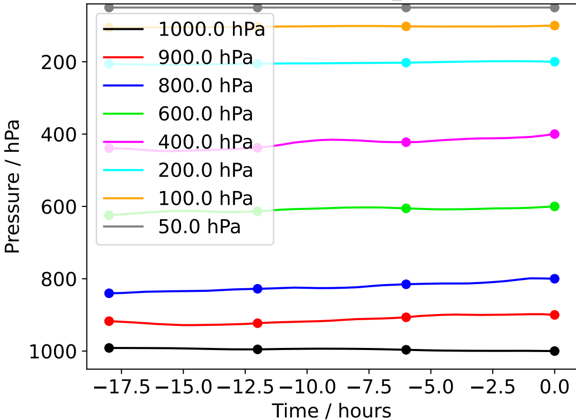
Camborne 20240213_180000
