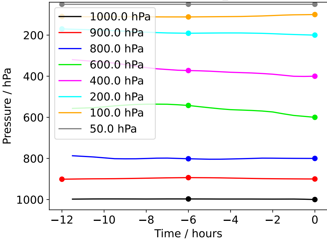
Camborne 20240122_120000
