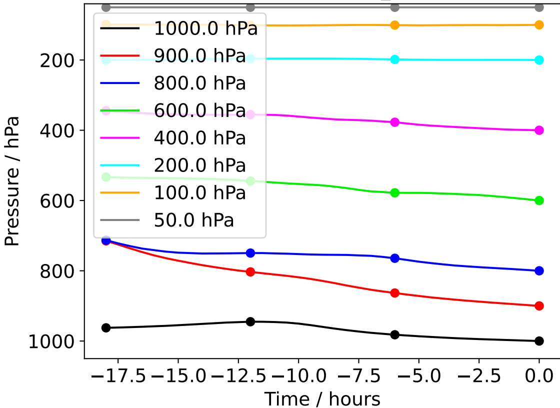
Camborne 20240118_000000
