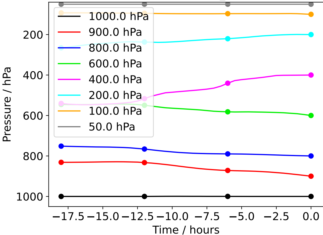
Camborne 20240117_000000
