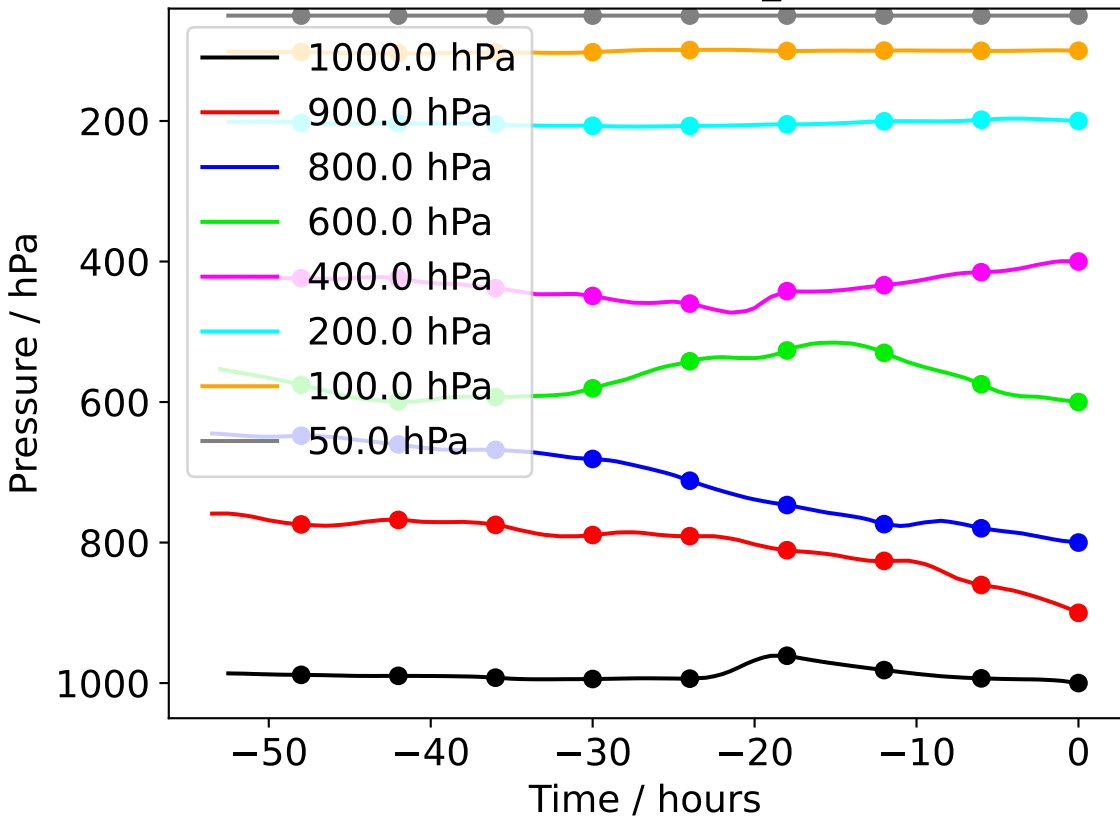
Camborne 20240105_000000
