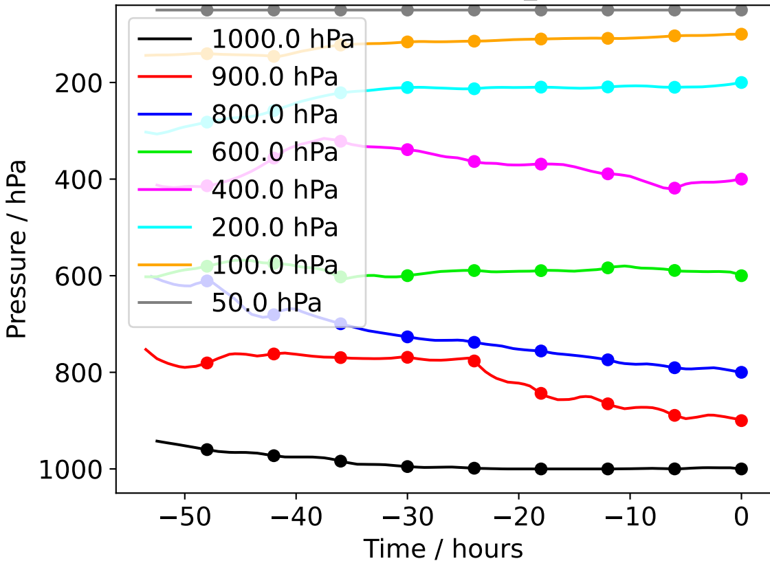
Camborne 20231228_180000
