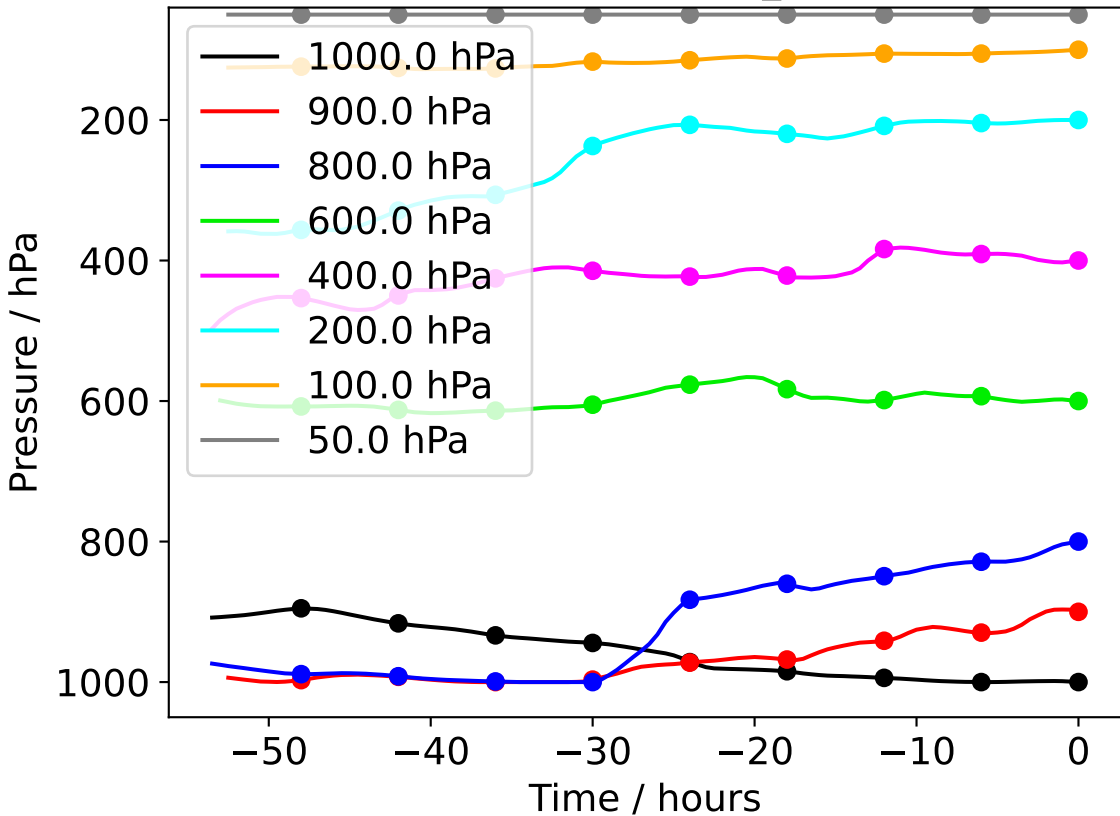
Camborne 20231225_060000
