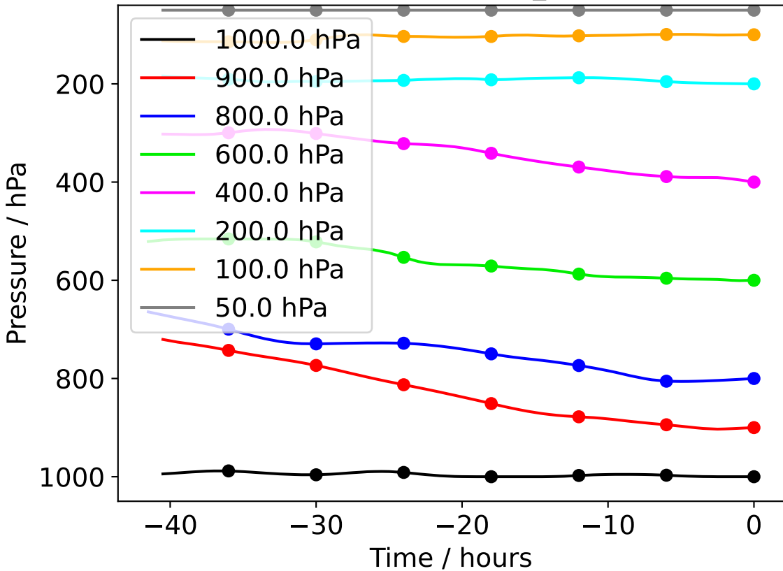
Camborne 20231217_060000
