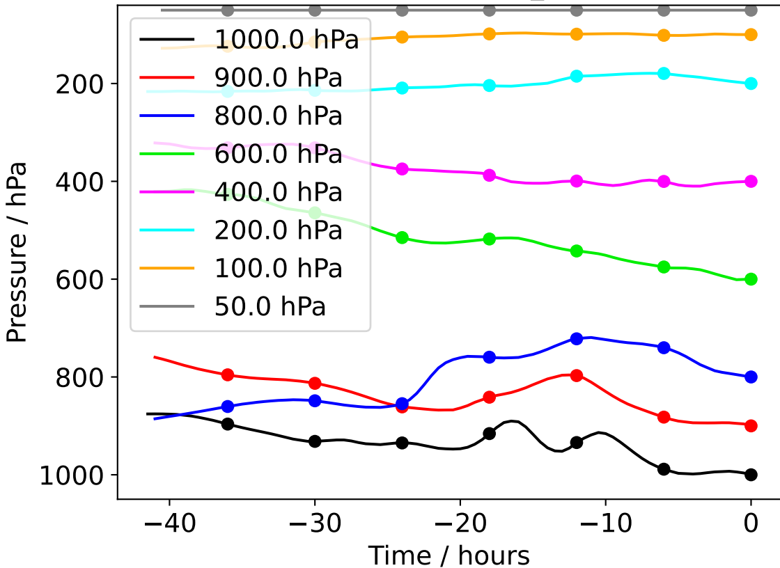
Camborne 20231213_120000
