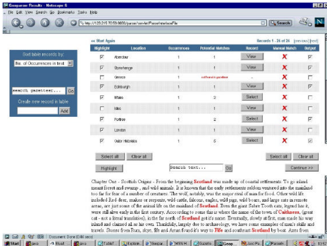
Fig. 4 An editing interface to the geoparser to assist in the semi-automatic georeferencing of documents.
