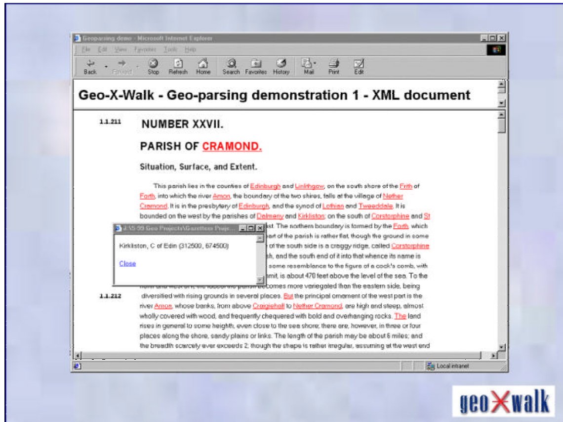
Fig. 3 A sample geoparsed document - underlined words have been automatically identified by the geoparser as potential placenames and where possible a georeference (OSGB National Grid coordinates) derived from the geoXwalk gazetteer.
