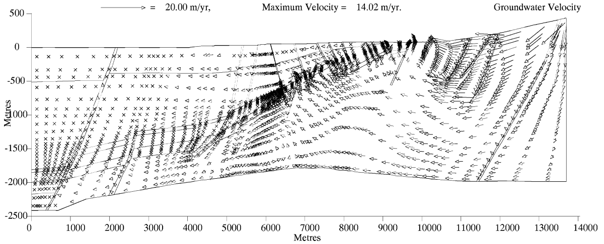
Fig. 8. Average linear velocities calculated with a complex model (Fig. 3). Model has faults and variable salinity profile. Hydraulic conductivities set to “base-case” (Table 1), except BVG (1.2 m year -1 ).
