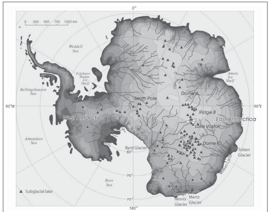
Fig. 1. The location of 145 known Antarctic subglacial lakes, ice-sheet surface elevation, and large-scale flow paths of subglacial water. Ice surface contours are in 500-meter intervals [from Siegert et al. , 2007].
