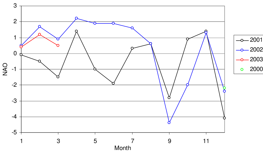
Figure 18. Monthly variation of NAO index for the time span relating to Figure 10. No data were available after March 2003. Data courtesy of J.W. Hurrell (Climate Analysis Section, National Center for Atmospheric Research, Boulder, Colorado, USA) - http://www.cgd.ucar.html .
