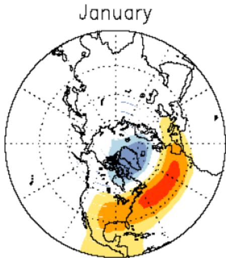
Figure 17. The Iceland Low pressure system and the Azores High pressure system; the driving forces of the NAO.
