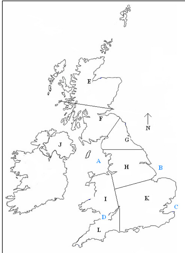
Figure 4. A map showing the British Isles split into zones. Maximum potential electricity production for each zone is shown in Table 2.
