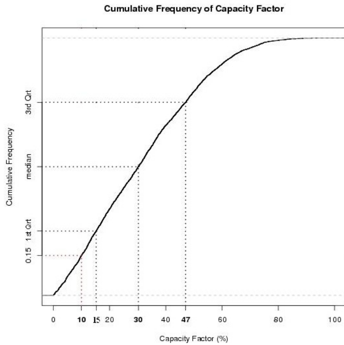
Figure14. Cumulative frequency of the capacity factor for UK wind power.
