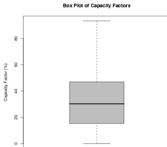
Figure 8. A box plot of the estimated, 6-hourly capacity factor data accounting for all wind power in the UK (future and present). The Black line shows the mean average, the two mid-quartiles are shown by the grey box (i.e. 50% of the time the CF lies within this range) and the maximum and minimum values are shown by the upper and lower bars.
