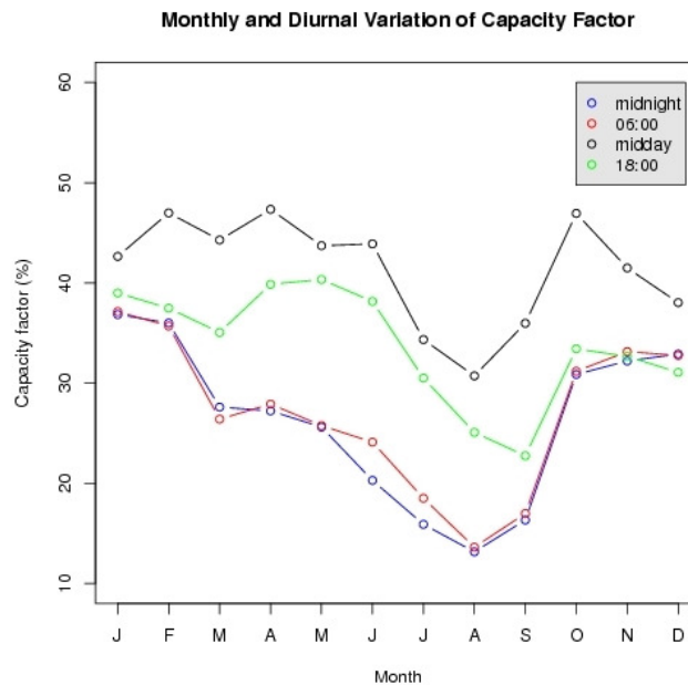
Figure 11. Diurnal fluctuations of CF for each month. Each line relates to a different time of the day according to the legend.
