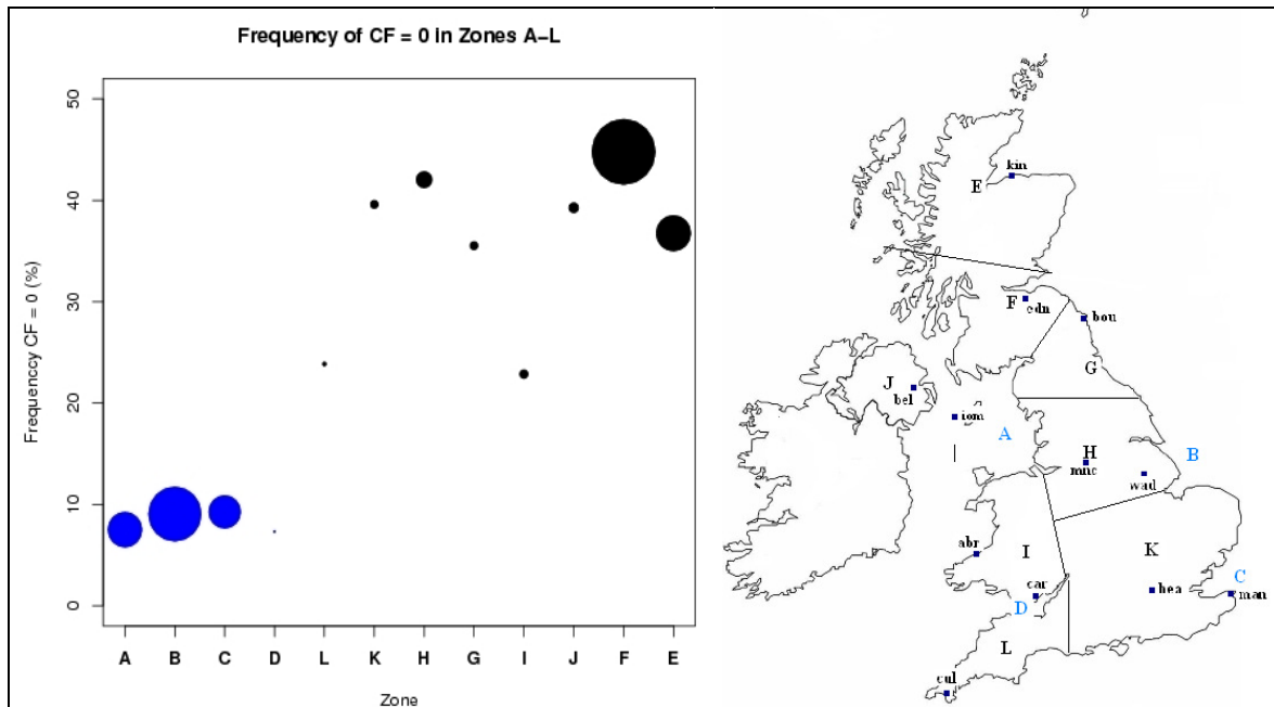
Figure 15. Percentage of time when power production is zero, for each of the 12 zones around the UK (shown on the right). The markers, sized proportionally to the amount of electricity being produced in that zone, are ordered with the offshore sites first (in blue), followed by the most southerly zone, moving north there after. For reference, the circle representing southern Scotland (zone F) equals 4 GW of electricity production.
