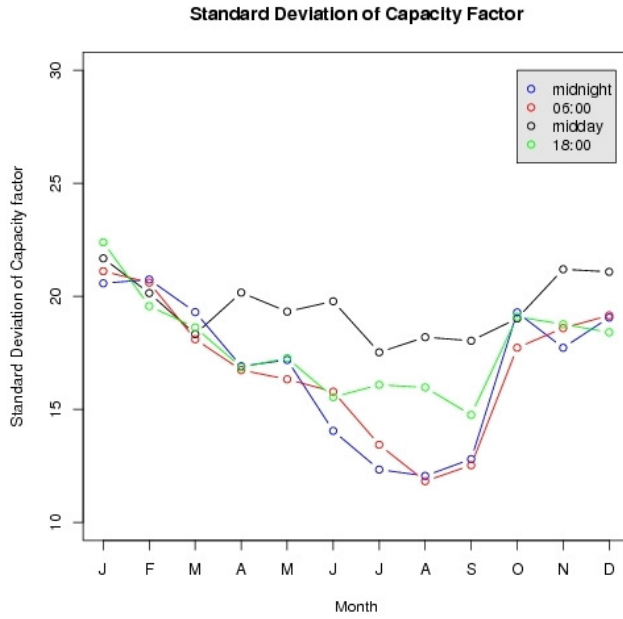
Figure13. Standard Deviation of CF shown for each time of the day in each month as per Figure 11.
