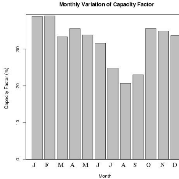
Figure 9. Average monthly CF for the British Isles wind power, averaged over a three year period.
