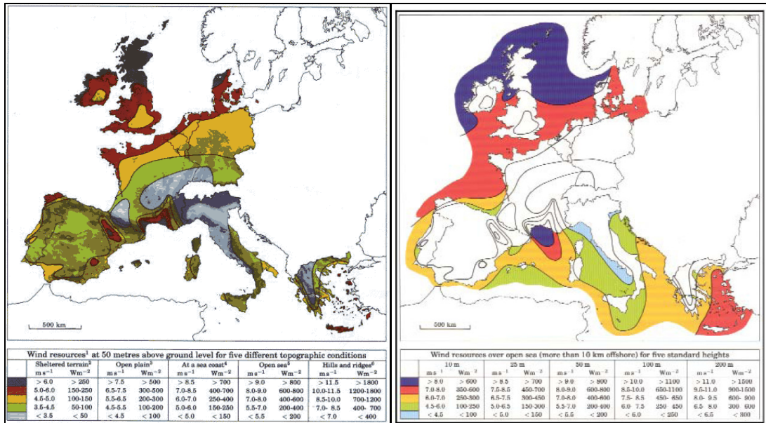
Figure 3. Maps showing distribution of average wind speeds around Europe. The British Isles and particularly Scotland are the windiest regions. Reproduced from Wind Power in the UK: a guide to the key issues surrounding onshore wind power development in the UK .
