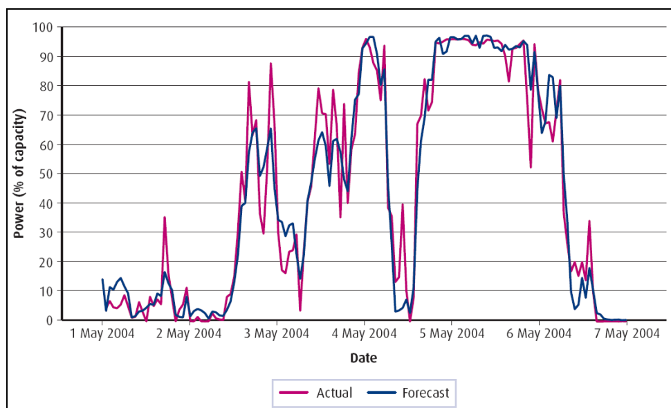
Figure 20. The forecast of power output from one wind farm given 1 hour in advance vs the actual power output, Ireland 2004. Reproduced from SDC, 2005.
