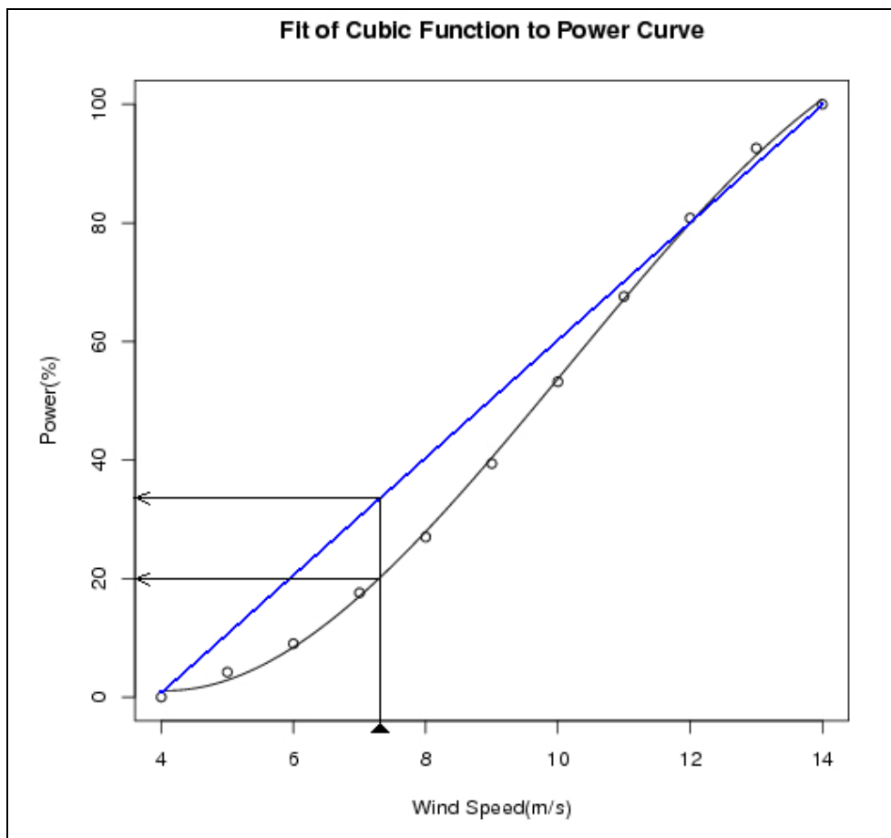
Figure 7. A plot showing the fit of the cubic function (2) shown by the black line, to some actual turbine data (circles). Also shown is the straight line (blue) initially used to model the power curve, and the difference between the two models at 7.68 \text{ms}^{-1} (the overall average wind speed). The R code written to compute the cubic co-efficients can be found in the appendix (7.2).
