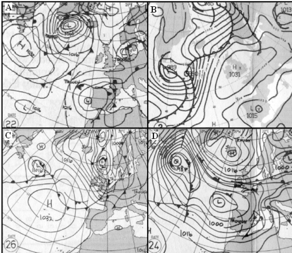
Figure 16 a-d. Barometric charts corresponding to: a & b – days of zero power production, c – the hour of maximum power production where UK wind farms would have theoretically been producing 93% of their potential, and d – an hour of 30 % power production. Charts are taken from the Royal Met Soc Journal called Weather , which is produced monthly.
