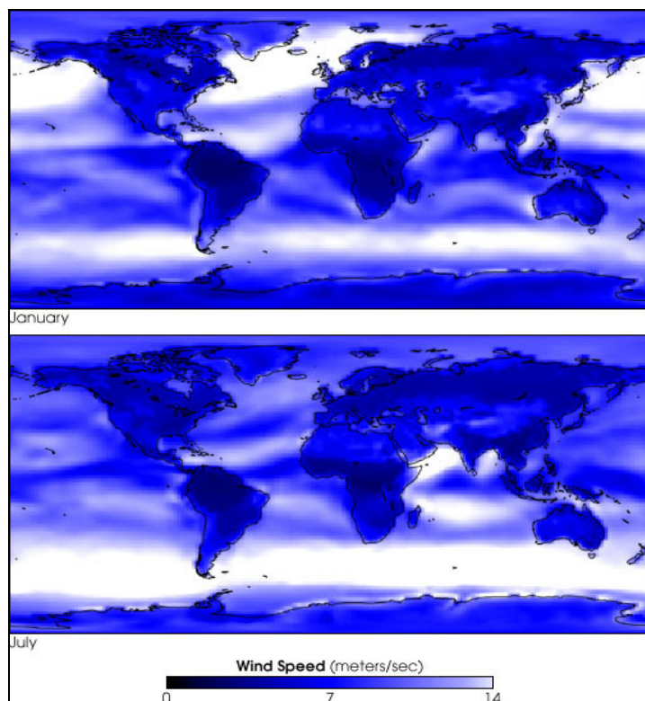
Figure 2. Maps showing global average wind speed data in mid-summer and mid-winter. Average wind speeds around the UK look favourable. Maps produced by Langley Research Centre, NASA.
