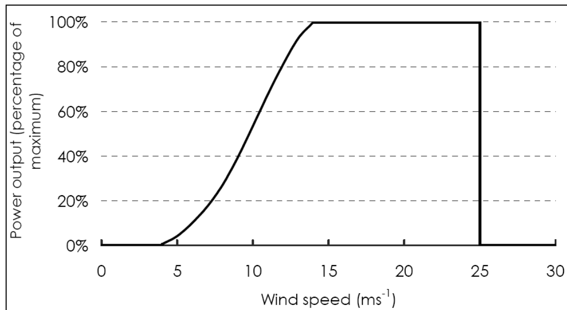
Figure 6. A typical power curve for a wind turbine. Reproduced from Sinden, 2005.
