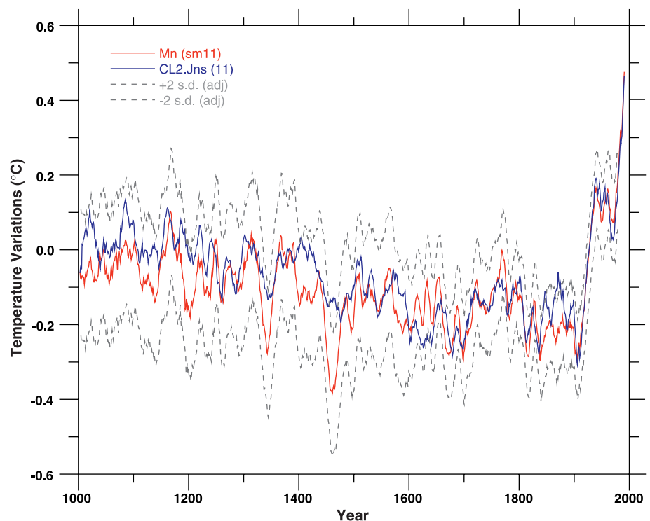
Fig. 1. Comparison of decadal smoothed Northern Hemisphere mean annual temperature records for the past millennium (1000–1993), based on reconstructions of Mann et al. (Mn) (17) and CL (12). The latter record has been spliced into the 11-point smoothed instrumental record (16) in the interval in which they overlap. CL2 refers to a new splice that gives a slightly better fit than the original (12). The autocorrelation of the raw Mann et al. time series has been used to adjust (adj) the standard deviation units for the reduction in variance on decadal scales.
