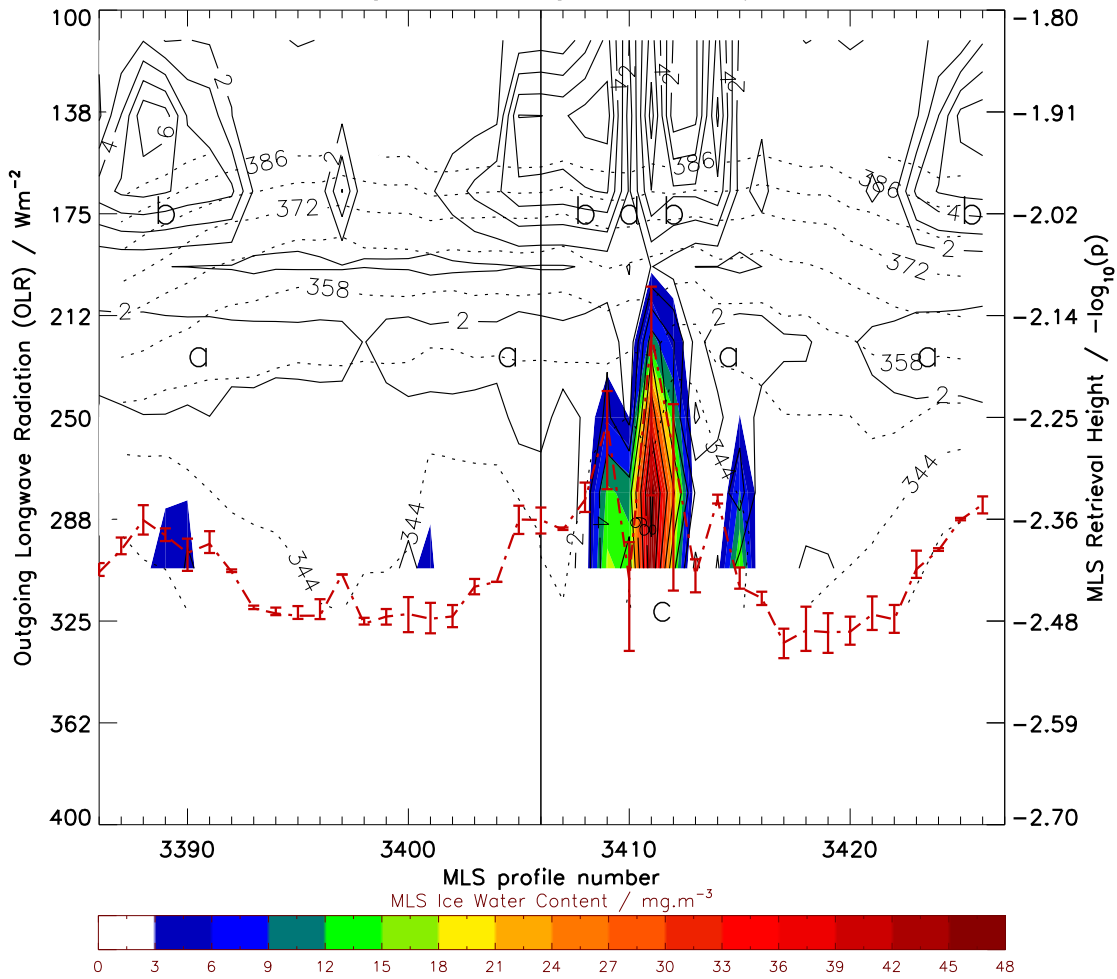
Plot of EOS MLS Cloud Ice Measurements and the associated Longwave Heating Rate / \text{Kday}^{-1}
