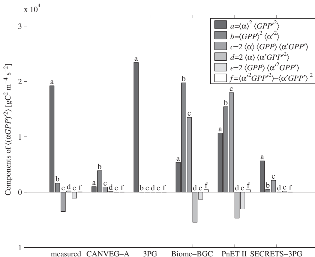
Fig. 8 Components of the expansion of \langle(\alpha GPP)^2\rangle for measurements and for each model.
