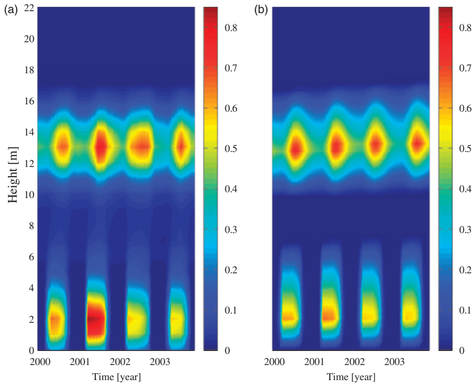
Fig. 2 Time-depth variations (color plots) of leaf area density ( LAD , m^2 m^{-3} ) as function of year and height from forest floor. (a) Field estimations of LAD . (b) LAD modeled by CANVEG with carbon allocation.
