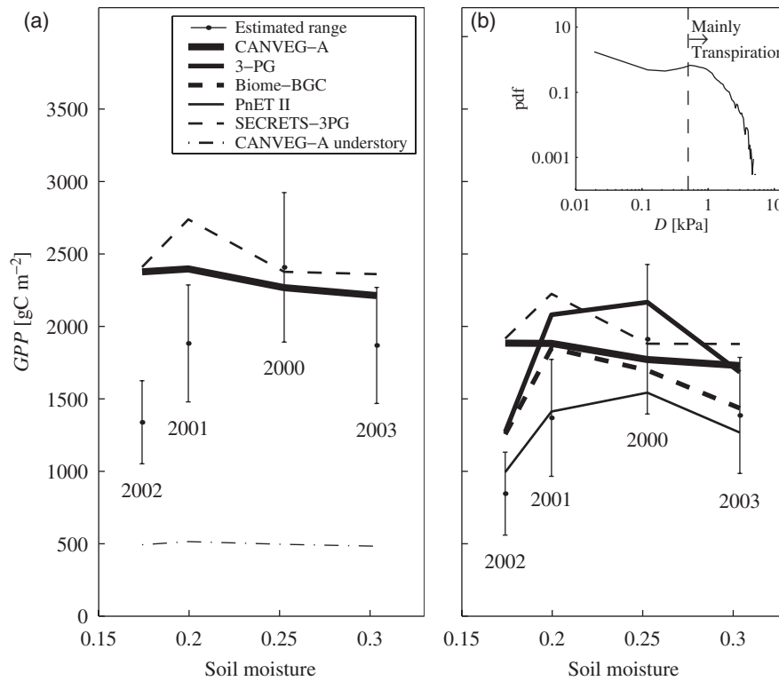
Fig. 6 Comparison between estimated gross primary production ( GPP ) and modeled GPP . The inset shows the pdf of vapor pressure deficit ( D ) on a log scale. The upper and lower GPP limits (vertical line) were computed assuming \hat{C}_i/C_a is represented by sunlit or shaded foliage, where \hat{C}_i/C_a is the vertically integrated ratio of intercellular to atmospheric \text{CO}_2 concentration. Panel (a) represents total GPP (pine + understory) and panel (b) represents pine GPP only. The estimated range of pine only GPP was calculated by subtracting CANVEG with carbon allocation modeled understory GPP from the total estimated GPP .
