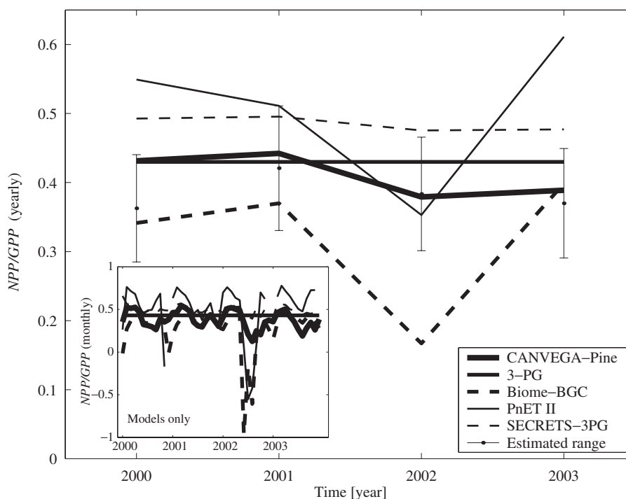
Fig. 7 Modeled net primary production ( NPP ) to gross-primary production ( GPP ) ratio. Note that physiological principles in predicting growth (3-PG) has a constant ratio shown as a straight line. The inset presents the monthly comparisons.
