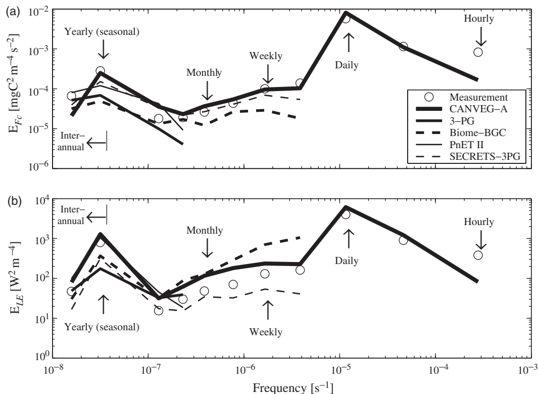
Fig. 4 Measured and modeled power spectra for the \text{CO}_2 flux F_c [panel (a)] and latent heat flux LE [panel (b)].
