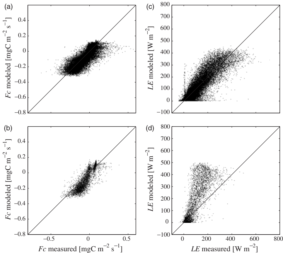
Fig. 3 Comparison of half-hourly CO 2 flux ( F c ) and latent heat flux ( LE ) measured by the eddy-covariance system and modeled by the CANVEG with carbon allocation (CANVEG-A). Panels (a) and (c) show no water stress runs in the 4-year period and panels (b) and (d) show runs during the drought period (April–September 2002). The 1 : 1 line is shown for reference.
