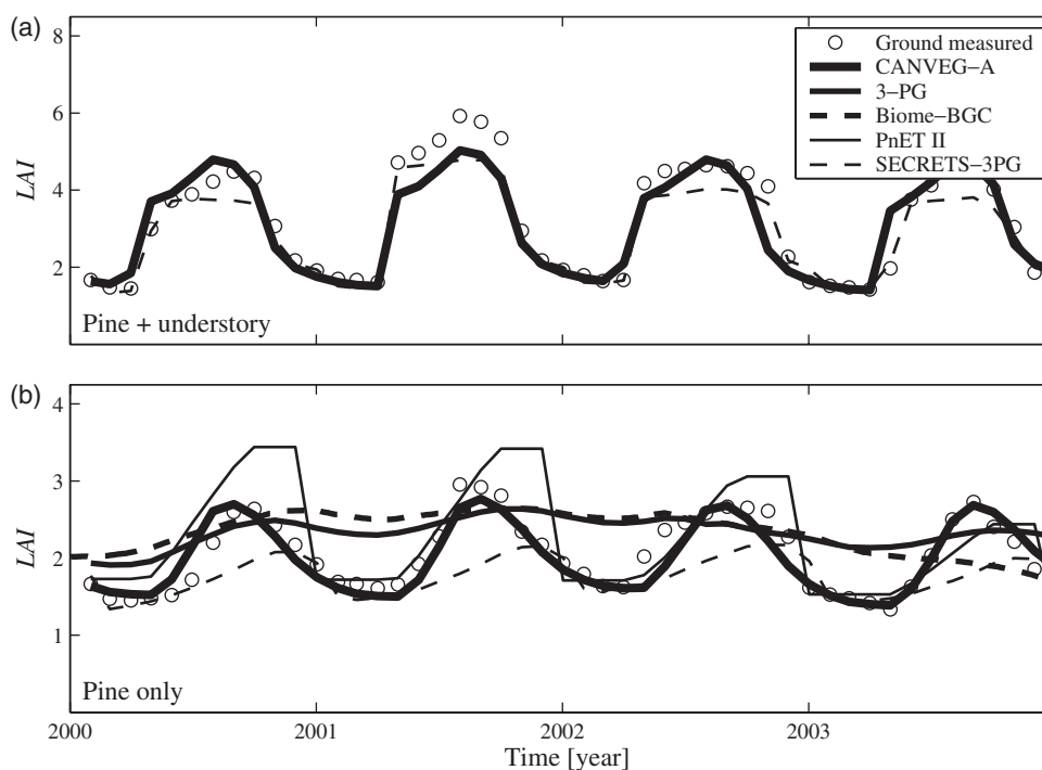
Fig. 5 Comparison between ground-based measured and modeled monthly time series of leaf area index (LAI). Panel (a) shows total LAI (pine and understory) and panel (b) Pine only LAI. Notice the different scale of the panels.
