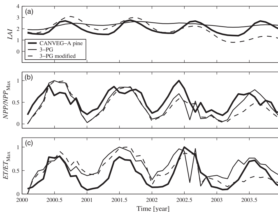
Fig. 1 Time series for pine leaf area index ( LAI ), normalized net primary production ( NPP ), and normalized evapotranspiration ( ET ) for the CANVEG with carbon allocation (CANVEG-A), the original physiological principles in predicting growth (3-PG), and 3-PG modified to include a new litterfall parameterization.
