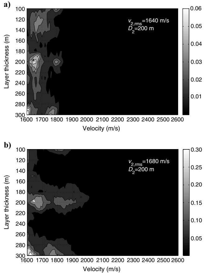
Figure 10. Spectra showing v_{2,rms} against D_2 . We assume that velocity increases with depth, and hence, we choose v_{2,rms} to vary from 1600 to 2600 m/s and increments every 10 m/s. The layer thickness D_2 spans from 100 to 300 m and increments every 10 m. We use a time window of 20 ms. (a) Semblance computed using all 400 sources in the correlation gather and for b_i = b_{k,j} = 2 in each layer. (b) As for (a) but using only the first 80 sources.
