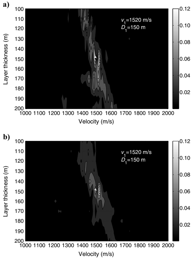
Figure 5. Spectra computed from the correlation gather in Figure 3a. The velocity v_1 spans from 1000 to 2000 m/s and increments every 10 m/s. The layer thickness D_1 spans from 100 to 200 m and increments every 10 m. We use a time window of 10 ms. In each of the following spectra we indicate the true value of velocity and layer thickness with an arrowhead and display the velocity-thickness pair with the highest signal coherency in the upper right-hand corner. (a) Semblance computed using all 400 sources and energy up to the first-order multiple ( b = 2 ). (b) As for (a) but computed using energy up to the third-order multiple ( b = 4 ).
